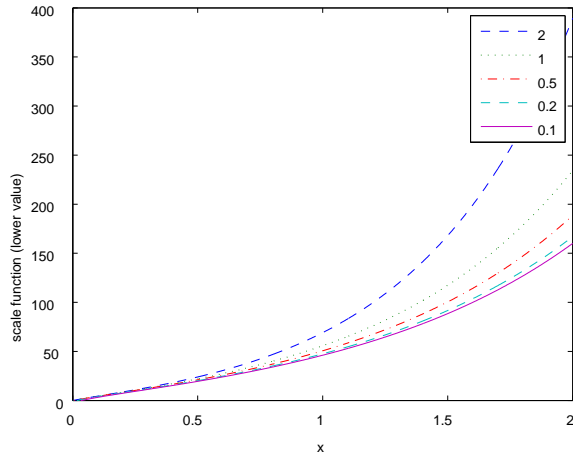
lower bounds for the scale functions
