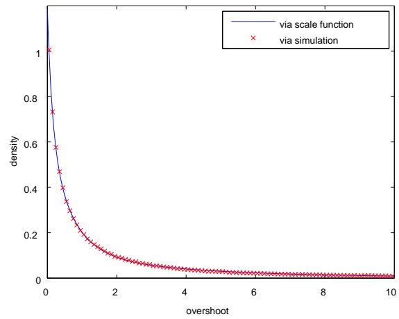
Pareto(1.2,5) with \sigma = 0
