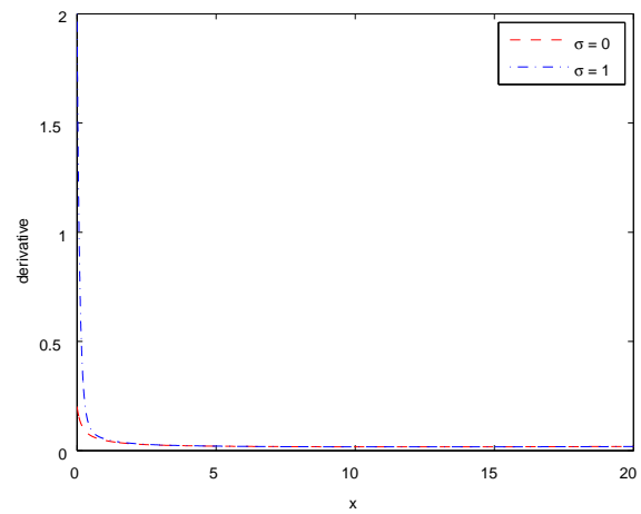
Derivative for the Pareto(1.2,5) case
