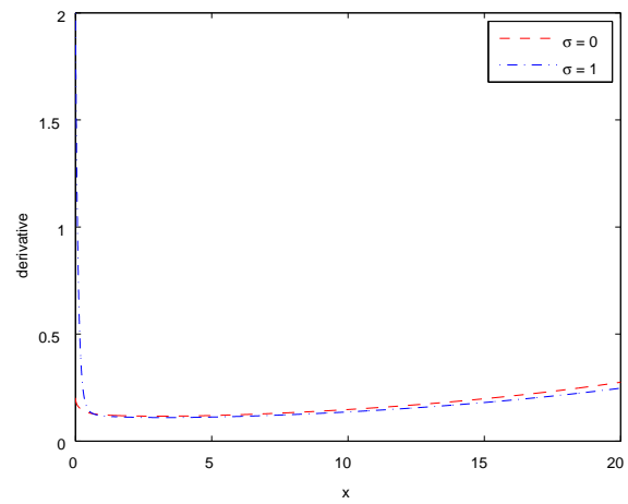
Derivative for the Weibull(0.6,0.665) case
