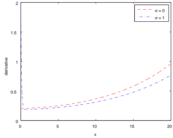
Derivative for the Exp(1) case
