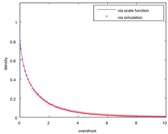
Weibull(0.6,0.665) with \sigma = 0
